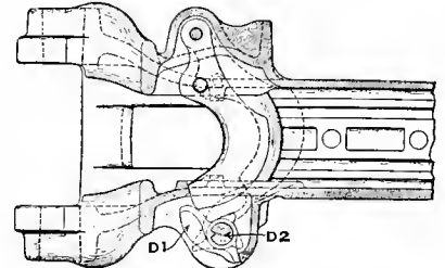
Fig. 2243. Sectional Plan, showing Swing Locks.
